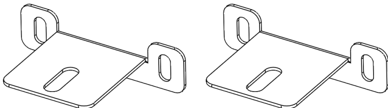
SURFACE MOUNT LIGHT BRACKET 2AFL2100-01 (x2)
